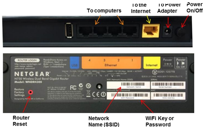
Figure 3 - NETGEAR N750 Router - Back Connection & Bottom Label Panels
